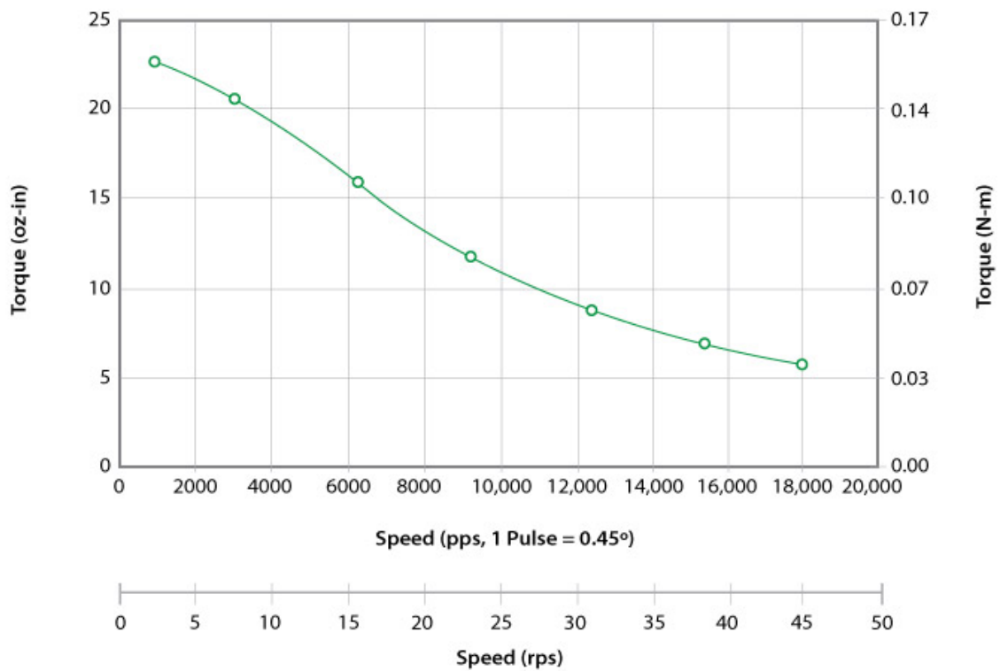
Z417-17-03 (0.9° Step Motor) 24VDC, 1.54 Amp Peak, Bipolar, 1/2 Stepping
